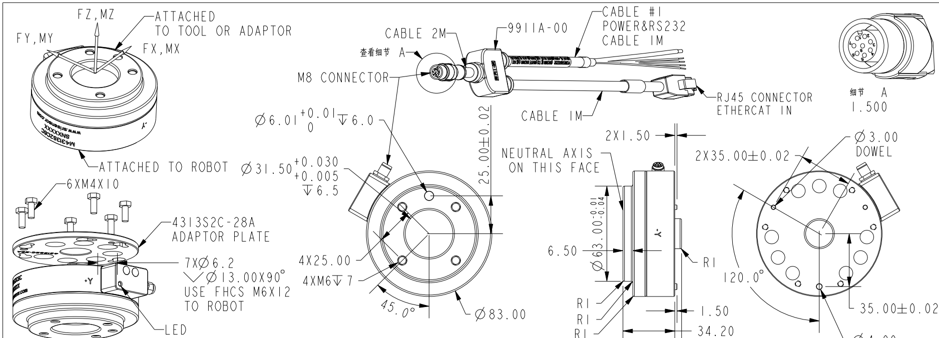
M8 CONNECTOR
